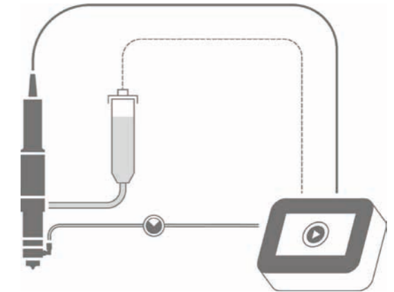
Non-self-levelling liquids, material to high viscosity material, incl. sensor technology and pressure feed
